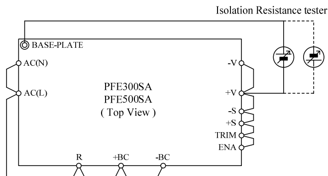
Fig. 6-7 Isolation Resistance Test Method
