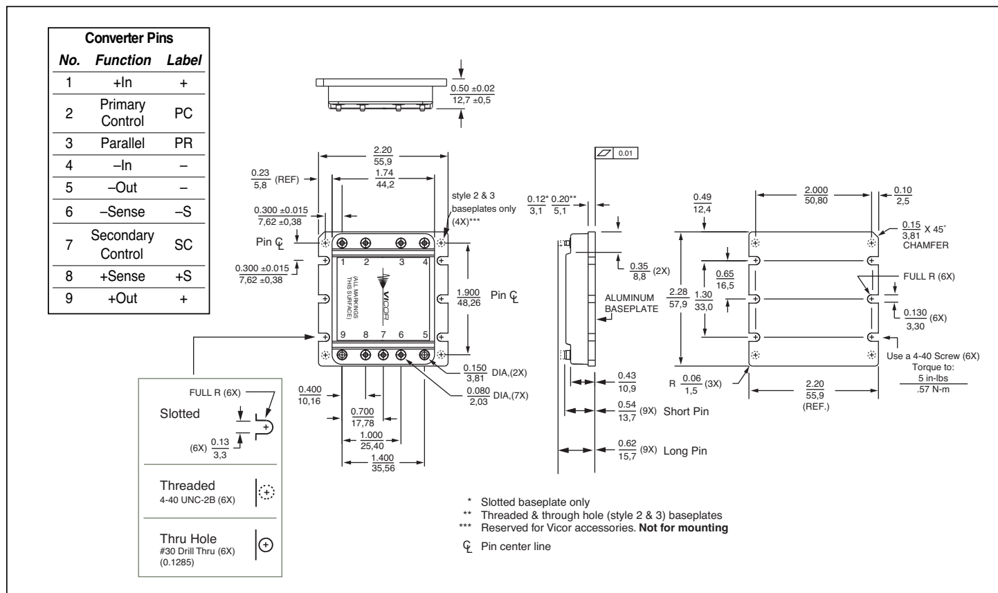
Figure 13 — Module outline
