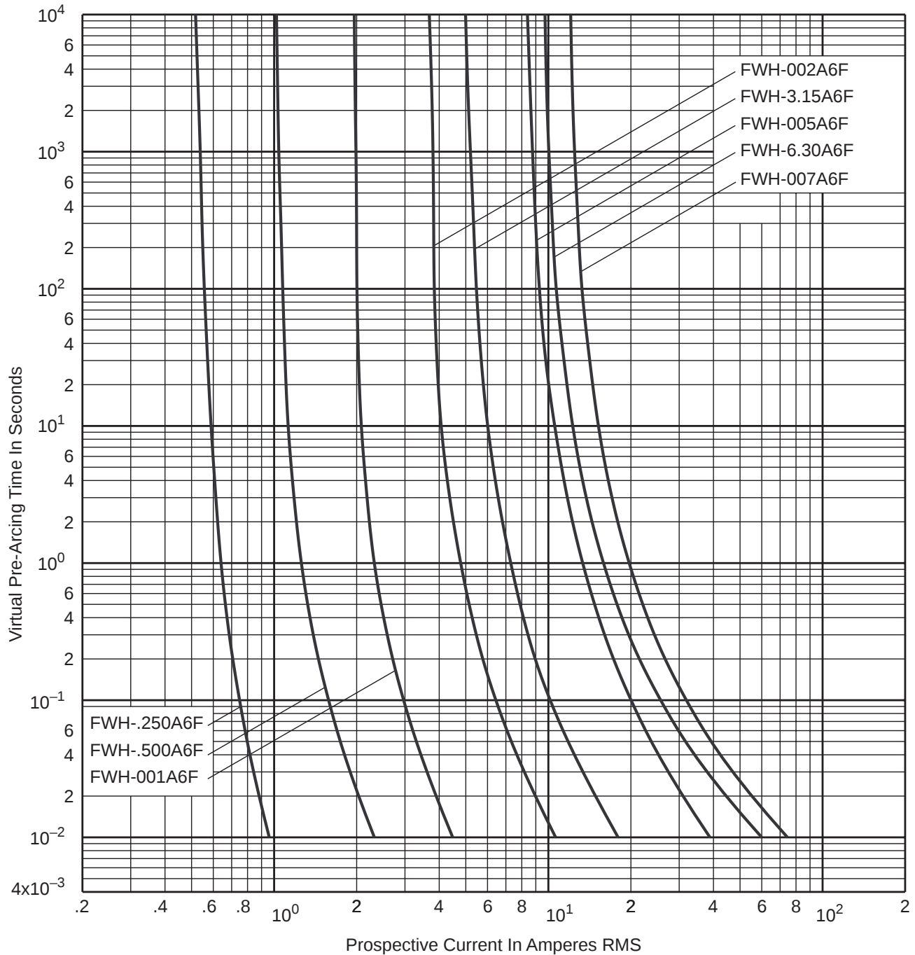
Pre-Arcing Time-Current Characteristic Curves FWH .250A6F-007A6F
