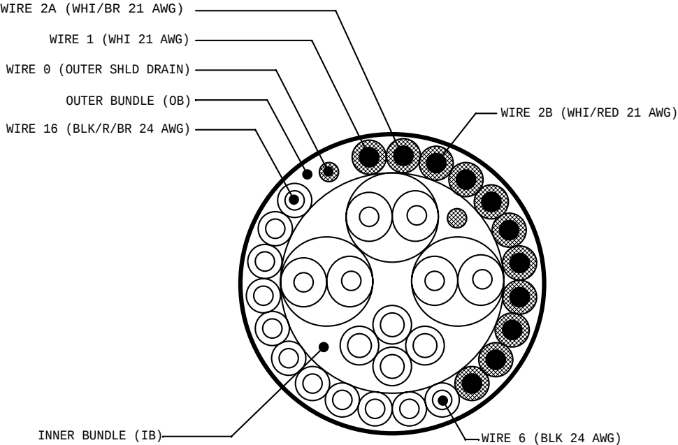
N23 CABLE LAYOUT
