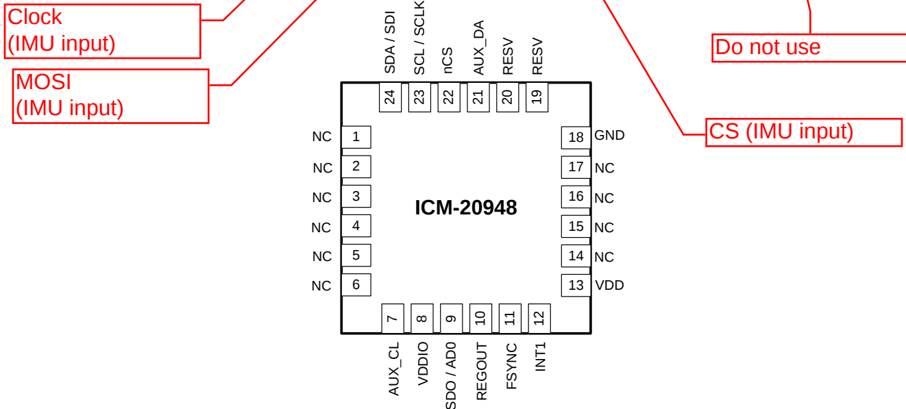
Figure 3. Pin out Diagram for ICM-20948 3 mm x 3 mm x 1 mm QFN
