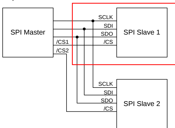
Figure 11. Typical SPI Master / Slave Configuration
