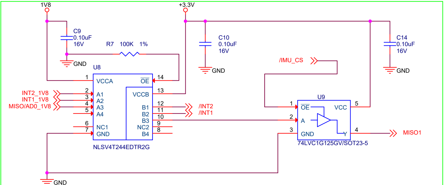
Level shifter 1.8V > 3.3V. This part is always-on. Output buffer enable MISO1 on /IMU_CS signal only
