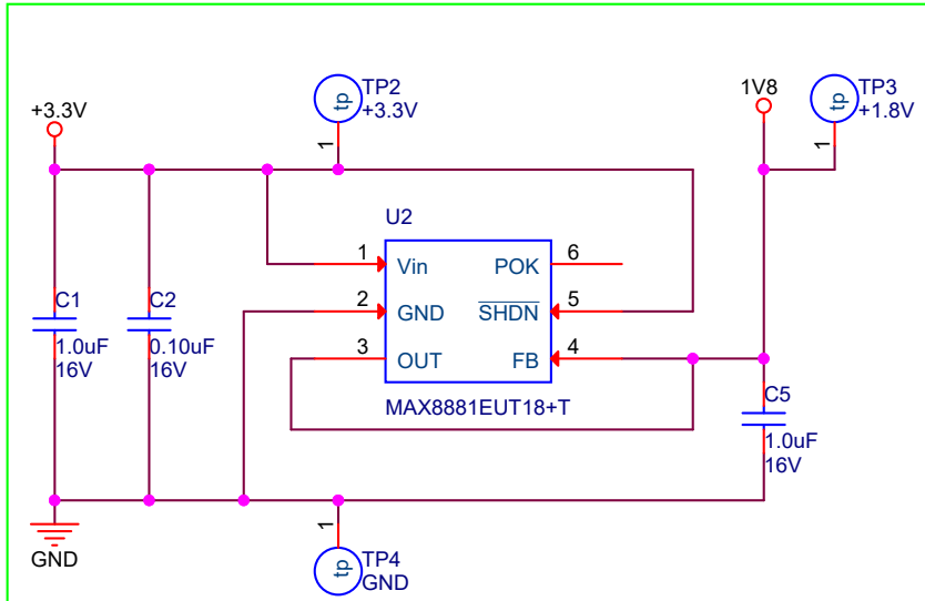
1V8 power, always ON
