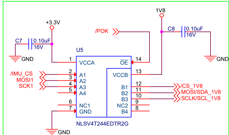
Level shifter 3.3V > 1.8V Always ON Outputs are controlled to tri-state when 1V8_SHDN goes to 90% of nominal
