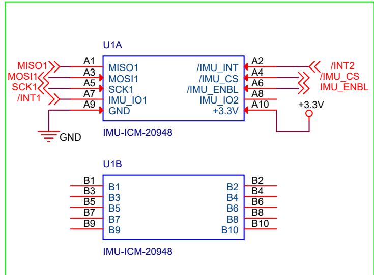
10020895-MOB3 interface connectors
