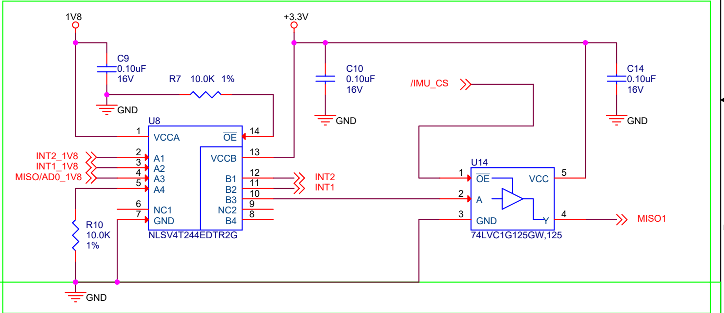
Level shifter 1.8V > 3.3V. This part is always-on. Output buffer enable MISO1 on /IMU_CS signal only
