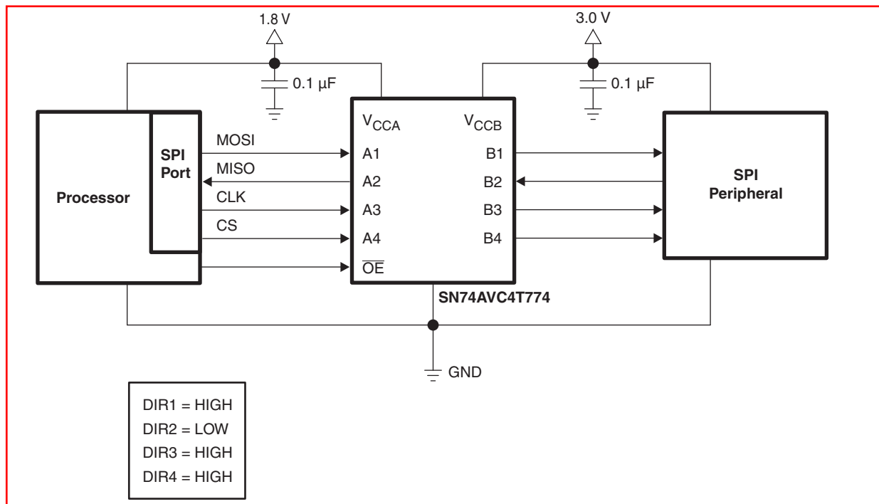
Figure 5. Typical Application of the SN74AVC4T774
