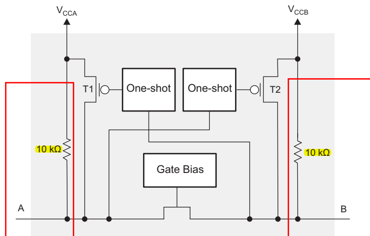
Figure 10. Architecture of a TXS01xx Cell
