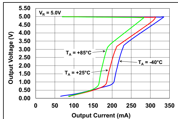
FIGURE 2-28: Output Voltage vs. Output Current.
