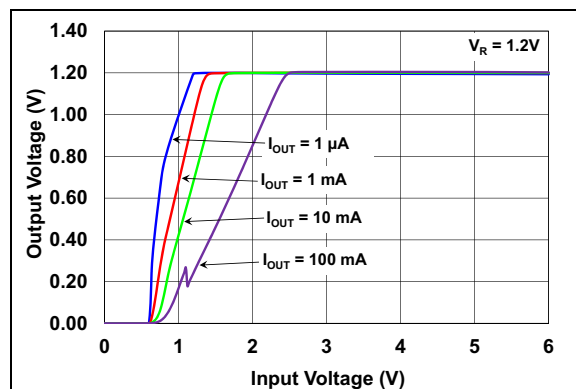
FIGURE 2-29: Output Voltage vs. Input Voltage.
