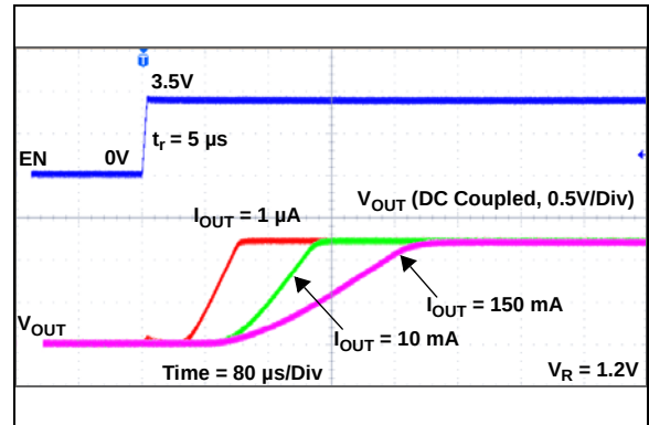
FIGURE 2-17: Start-Up from SHDN .
