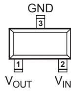
3-Lead SOT-23/SC70
