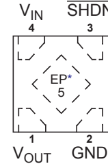
4-Lead 1x1 mm UDFN
