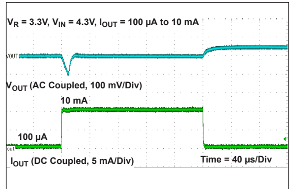
FIGURE 2-24: Dynamic Load Step (MCP1811X, V_R = 3.3\text{V} ).
