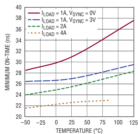
Minimum On-Time
