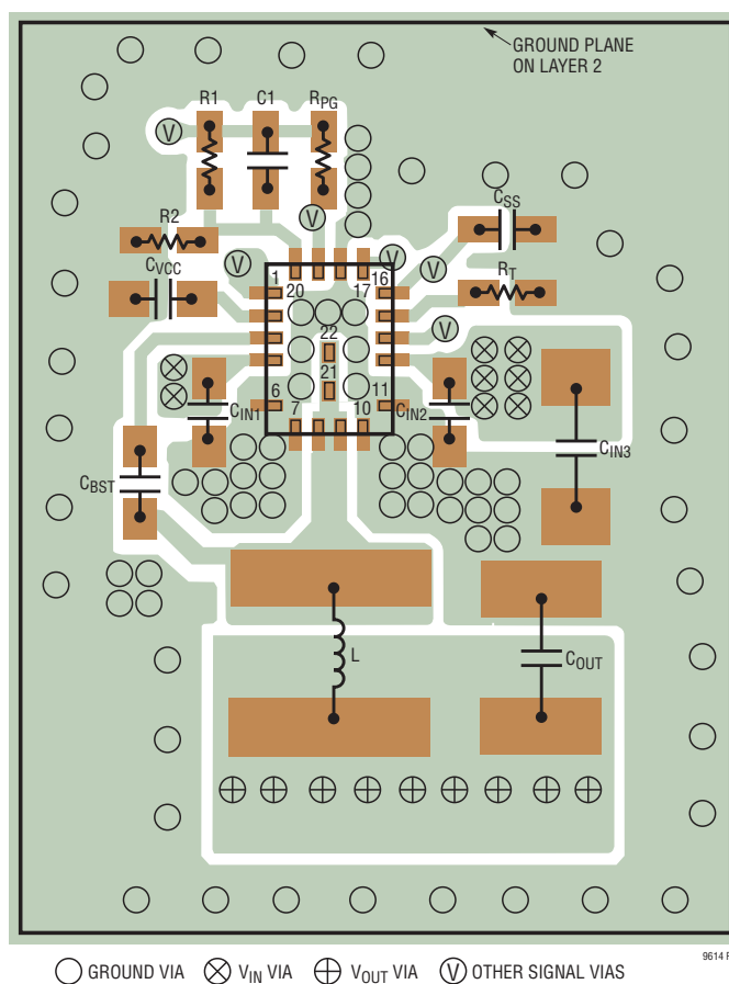
Figure 1. Recommended PCB Layout for the LT8614
