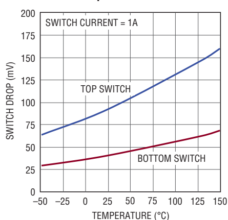
Switch Drop
