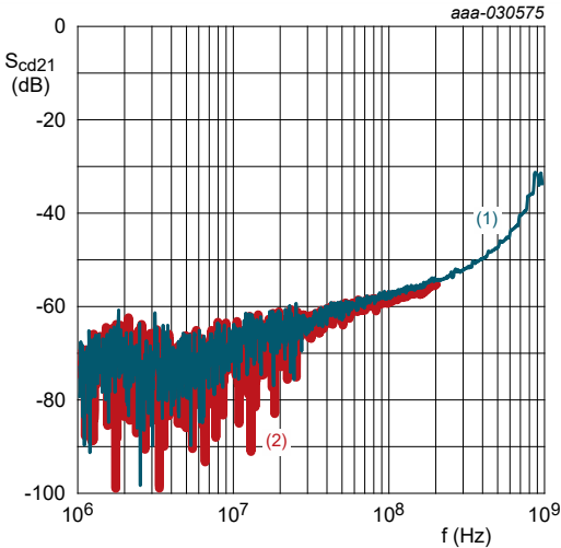
PESD2ETH100-T (1) before repetitive ESD event (2) after 20 times \pm 8 kV ESD
