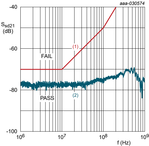
(1) limit according to OPEN Alliance 100BASE-T1 specification (2) PESD2ETH100-T
