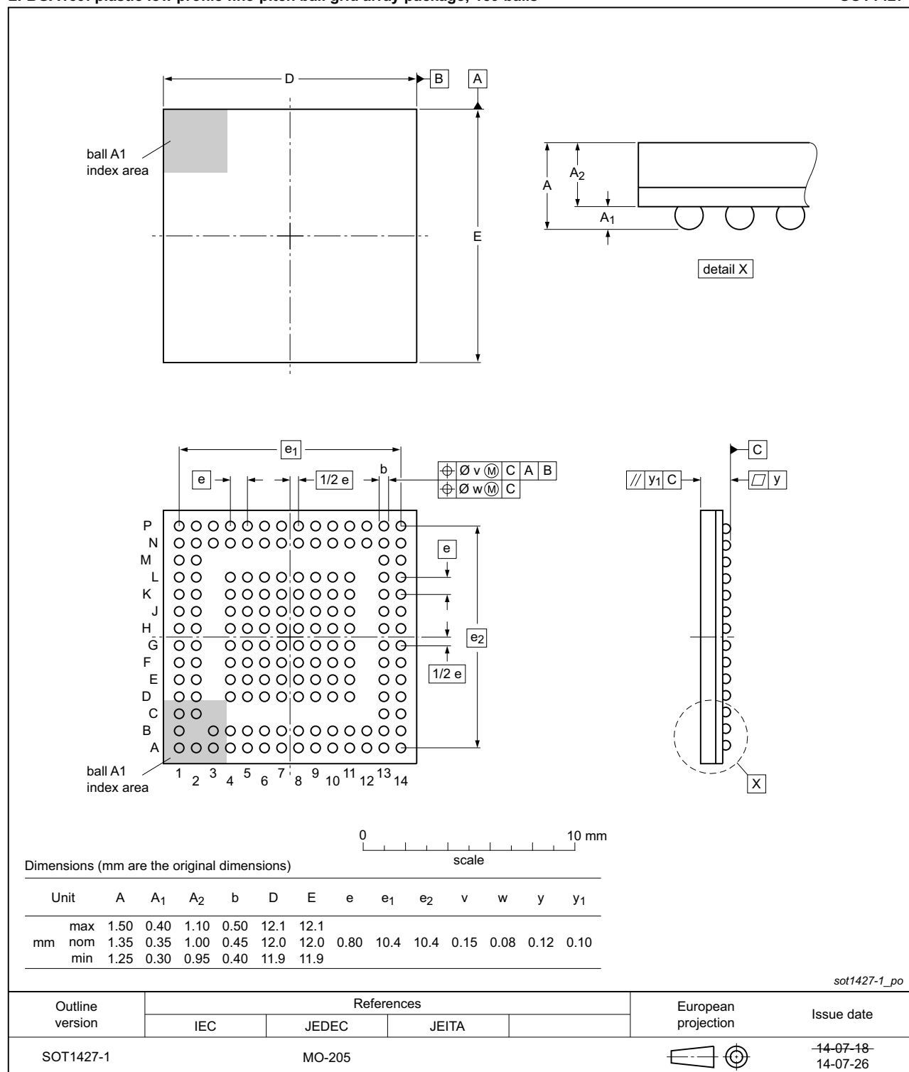
Fig 17. Package outline SOT1427-1 (LFBGA159)
