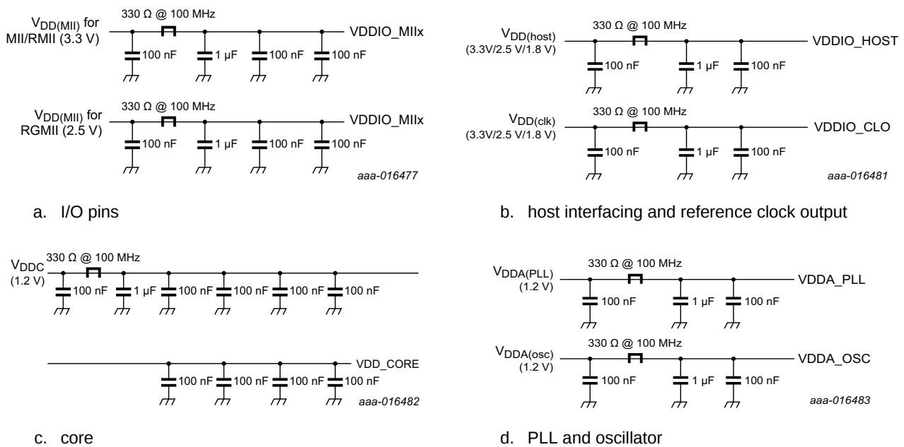
Fig 15. Power supply filtering
