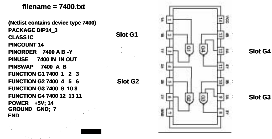
Figure 2-8 Device File Example
