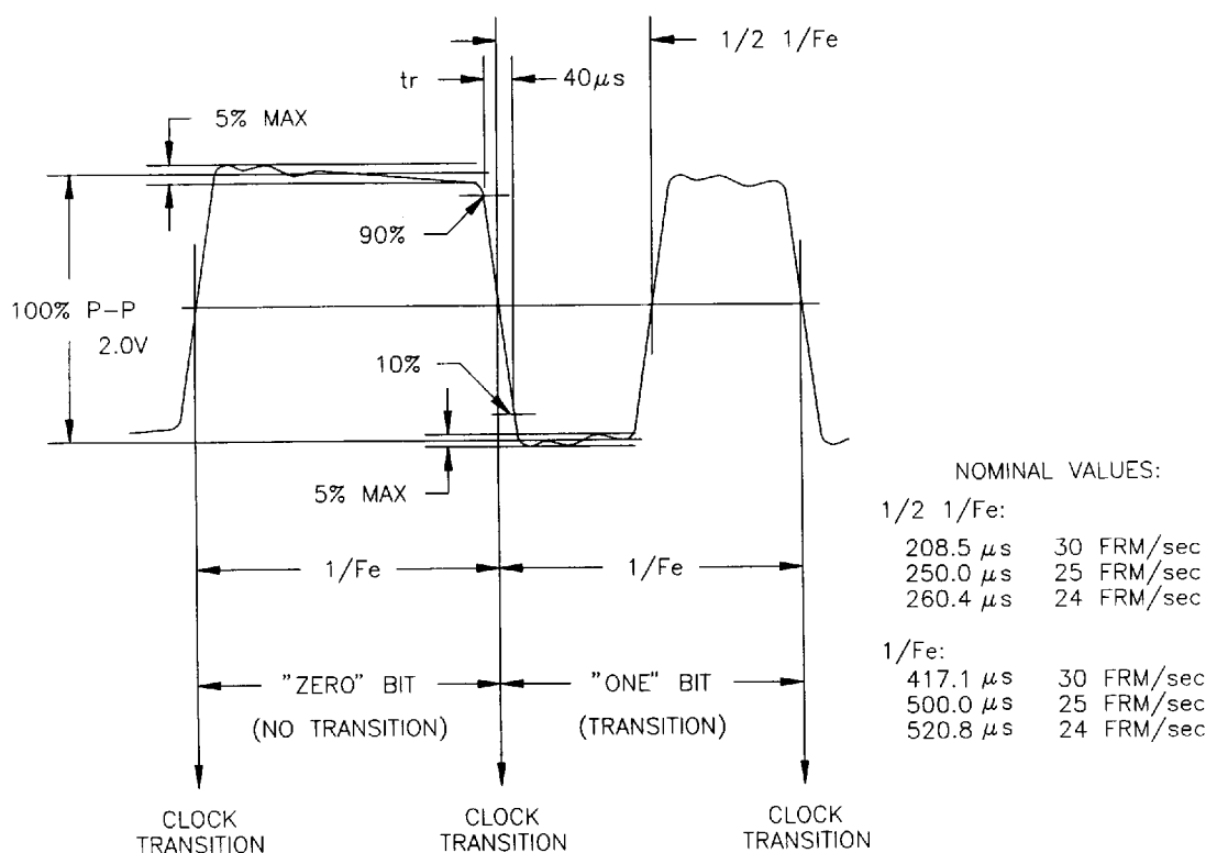
Figure 1 – Linear time code source output waveform
