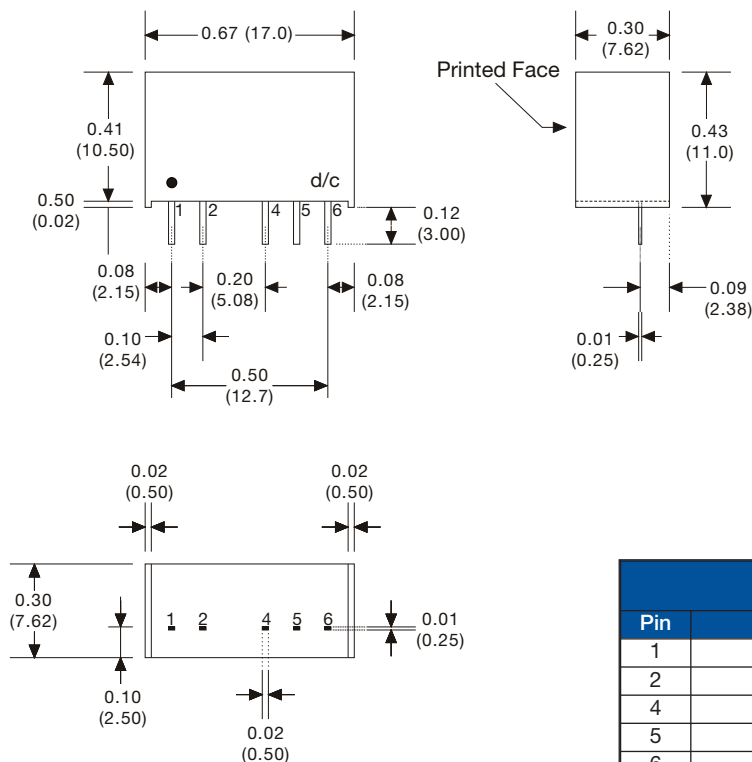
Pin Connections
