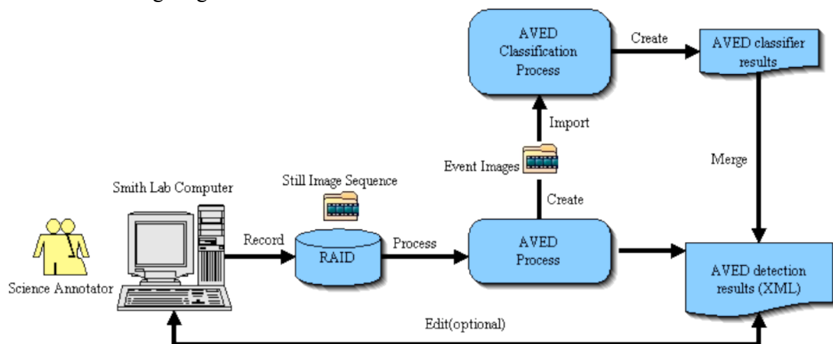
Figure 1. Data flow
