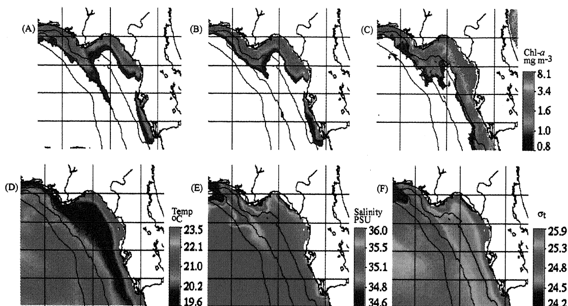
Figure 22. Simulated chlorophyll stocks at (a) surface and (b) middepth in relation to (c) composite SeaWiFS imagery and surface (d) temperature, (e) salinity, and (f) density fields of the circulation model during March 1998. The color codes of Figures 22a, 22b, and 22c are the same.
