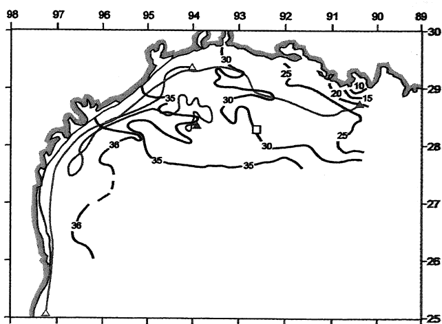
Figure 20. The near-surface distribution of salinity during the LATEX survey of 26 July–8 August 1993 in relation to the daily trajectories of holey-sock drifters [Howard and DiMarco, 1998] set at nominal depth of \sim 6 m on the inner shelf in November 1992 (red solid and open triangles) and on the outer shelf in May 1993 (green solid and open triangles). The same surface salinity of \sim 29.68 was found on the outer shelf (open square) in July 1975 [Reid, 1984].
