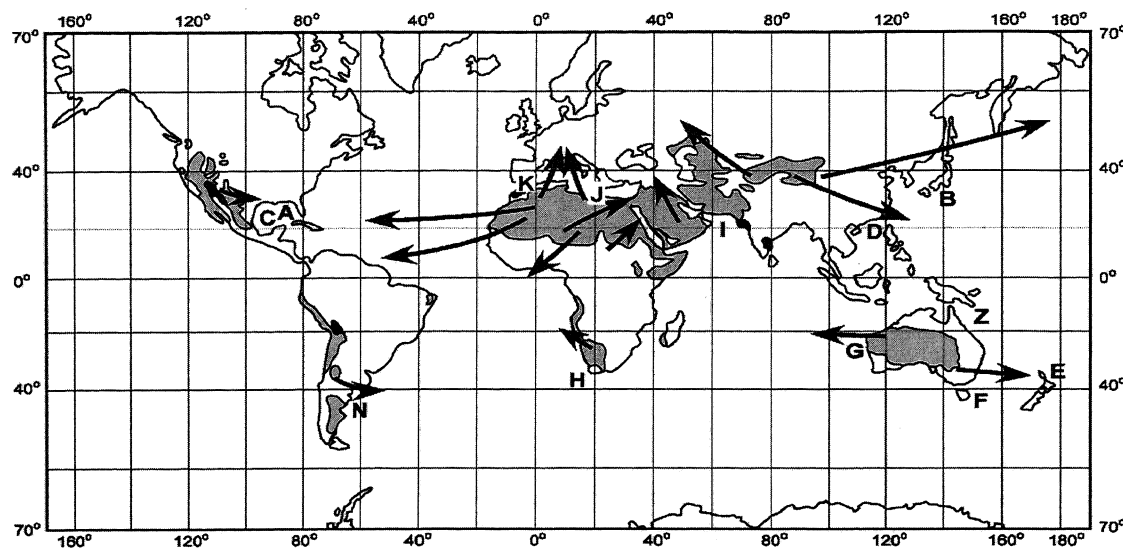
Figure 1. Locations of the Saharan, Saudi Arabian, Gobi, Simpson, Great Western, Kalahari, Atacama, and Patagonian Deserts and their downstream trajectories of aeolian dust [after Meigs, 1953; Pewe, 1981] in relation to red tides of Karenia brevis/mikimotoi off Florida (A) and Japan (B) over the last century, and off Texas (C), Hong Kong (D), New Zealand (E), Tasmania (F), Western Australia (G), South Africa (H), Kuwait (I), Greece (J), and Tunisia (K), over the last decade. The Argentine shelf (N) may have recent undetected red tides of Karenia , since Trichodesmium blooms and dust hazes prevail here, as well, while blooms of Karenia have been found off southern Chile. The Great Barrier Reef (Z) represents the null case of background populations of Trichodesmium , without dust influxes and low residual phosphate stocks, that yield small blooms of other dinoflagellates, instead of red tides of Karenia .
