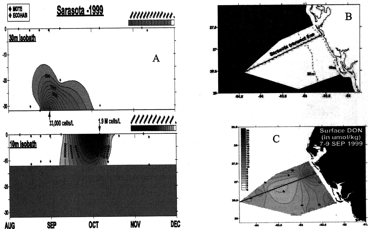
Figure 14. The (a) weekly distributions of Karenia brevis above the 30-m and 10-m isobaths during August–December 1999 of (b) the Sarasota, FL transect in relation to (c) surface DON stocks ( \mu\text{mol kg}^{-1} ) during September 1999, when the nitrate stocks were then <0.3 \mu\text{mol NO}_3 \text{ kg}^{-1} over the water column. The sampling interval was \sim 7 days ( www.floridamarine.org ), but only the occasions when K. brevis were present ( >1000 \text{ cells l}^{-1} ) are shown in Figure 14a.
