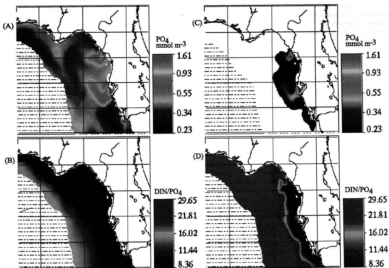
Figure 25. Simulated surface phosphate stocks and molar DIN/PO 4 ratios during August 1998, in response to (a and b) upwelling and outwelling sources, and (c and d) only estuarine supplies.
