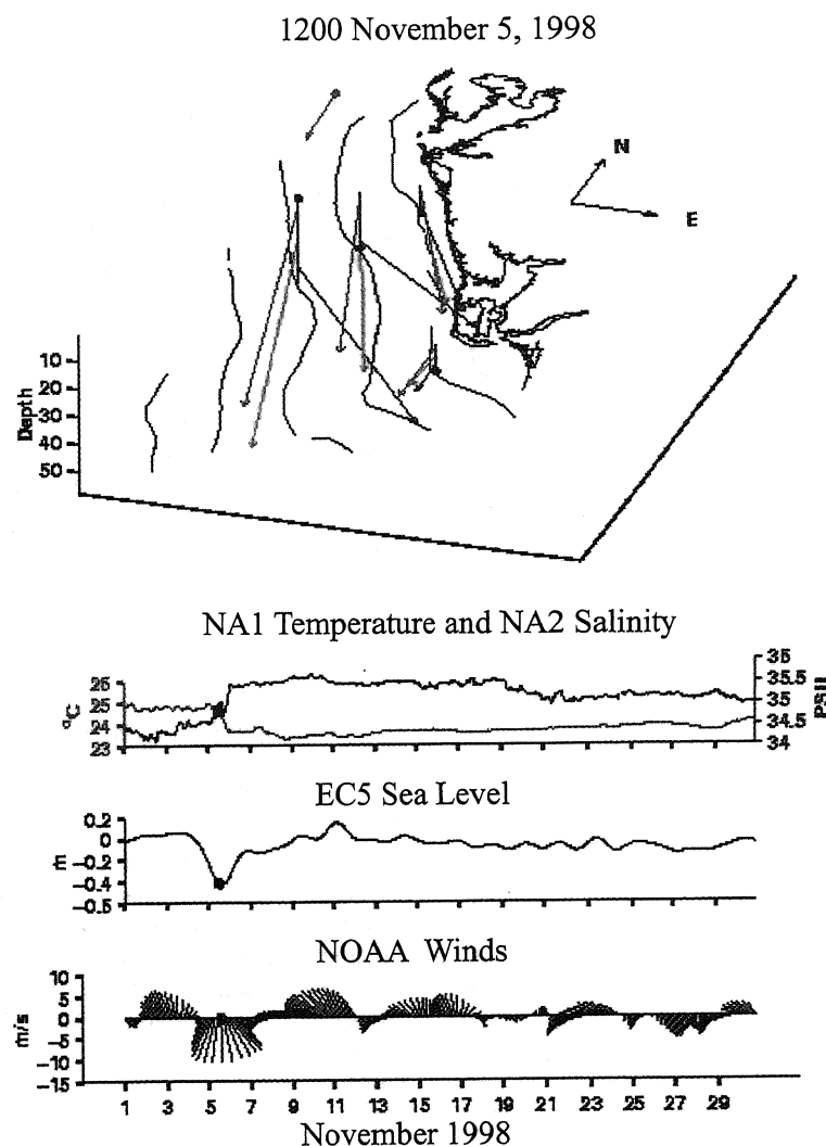
Figure 18. The three-dimensional current structure at noon on 5 November 1998 at the ECOHAB/HyCODE moored arrays, in relation to daily records of wind forcing at the NOAA offshore buoy, temperature and salinity at the 25-m isobath of the Sarasota, FL transect, and sea level at St. Petersburg, FL, during November 1998. The red, green, and blue colored vectors denote near-surface, middepth, and near-bottom flows.
