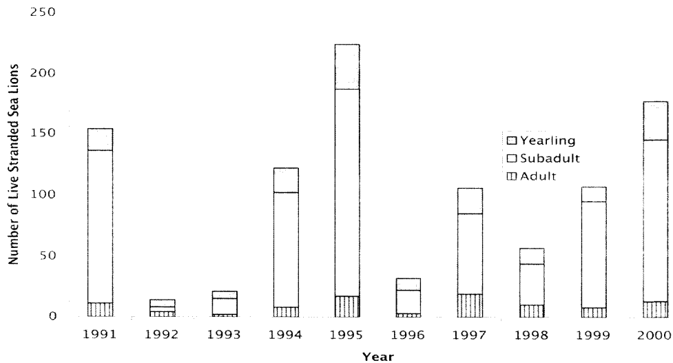
Figure 6. Age class of live California sea lions stranding with leptospirosis by year, 1991-2000
