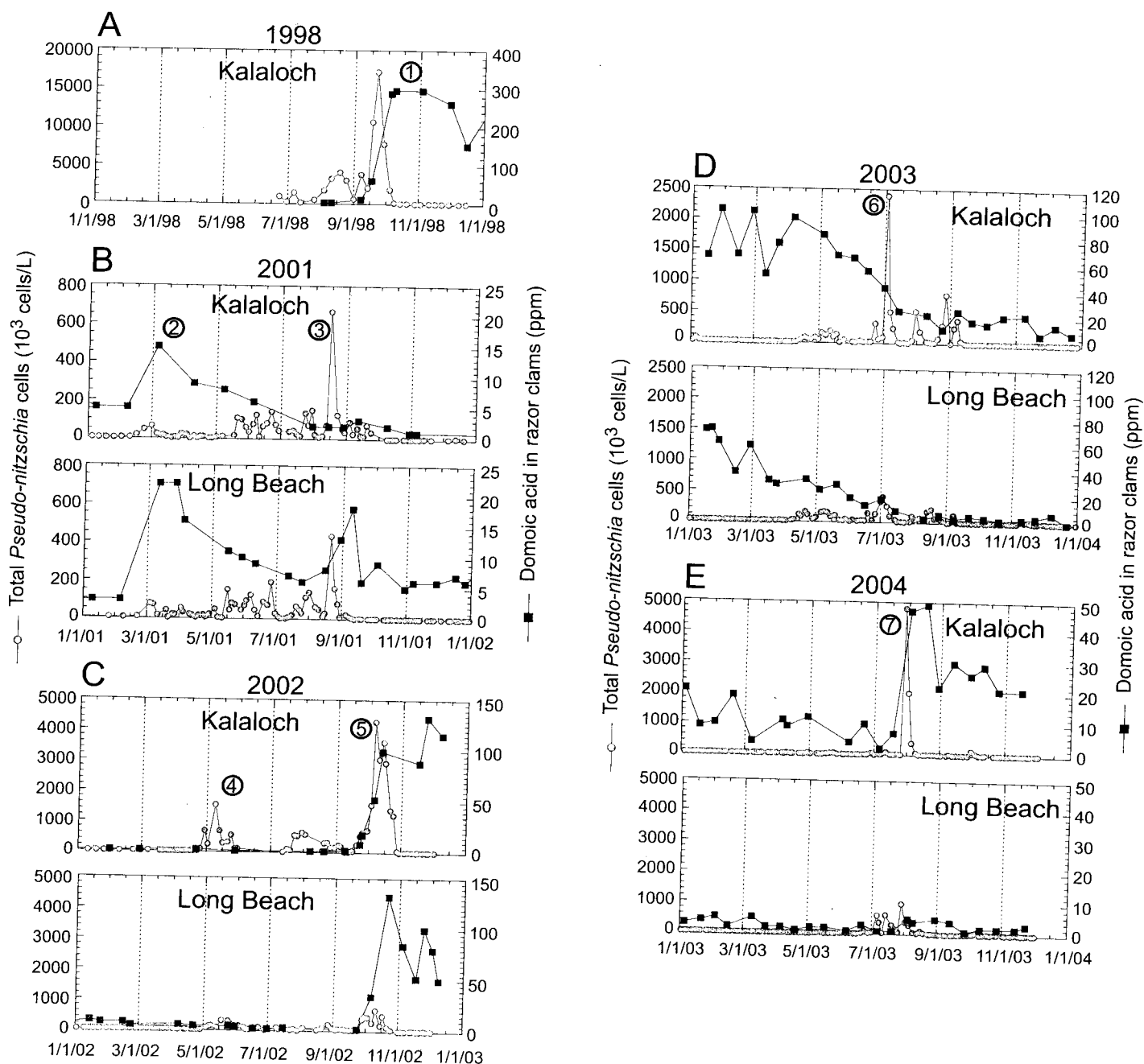
Figure 2. Pseudo-nitzschia cell numbers and domoic acid (DA) in razor clams at Kalaloch (1998, 2001 to 2004) and Long Beach (2001 to 2004) in Washington State. Identification and enumeration of Pseudo-nitzschia species present during each event were used to determine threshold levels of each size group that will trigger toxin testing in future samples. These events were used to determine threshold levels of Pseudo-nitzschia size groups that will trigger toxin testing: at least 3 \times 10^4 cells/L for P. australis/heimii/fraudulenta (short and broad), at least 1 \times 10^6 cells/L of P. cf. pseudodelicatissima/delicatissima (small and narrow) for a minimum of one week, and 1 \times 10^5 cells/L for P. multiseries/pungens (long and narrow). The rapid testing of domoic acid in seawater will allow managers to assess the total toxicity of a Pseudo-nitzschia assemblage and thereby determine the potential for toxin transfer to shellfish.
