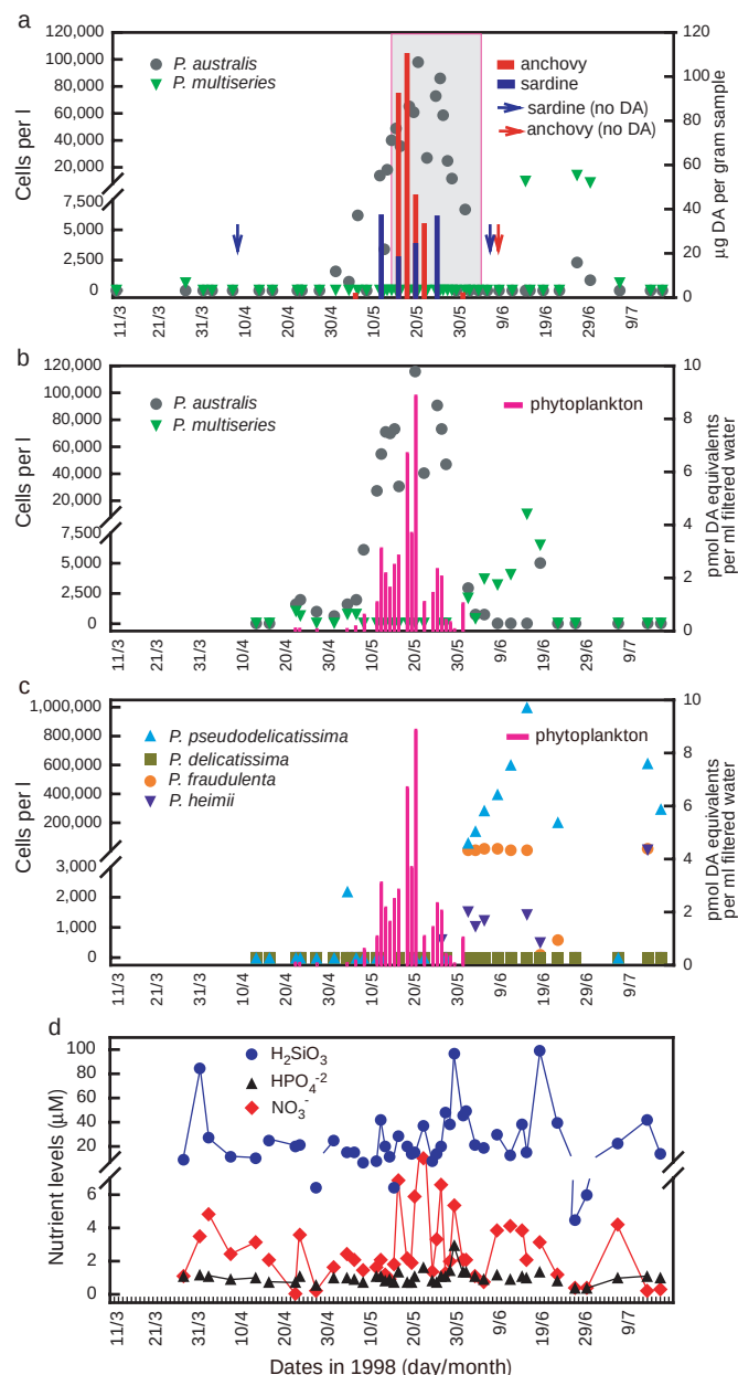
Figure 1 Abundance of Pseudo-nitzschia species, DA activity in plankton and fish, and nutrient concentrations. Data taken at Santa Cruz wharf from 11 March–16 July 1998.
