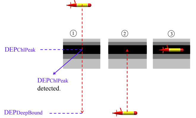
Fig. 2. Illustration of the algorithm for autonomous detection of the peak-chlorophyll layer, and drifting and sampling in the layer.
