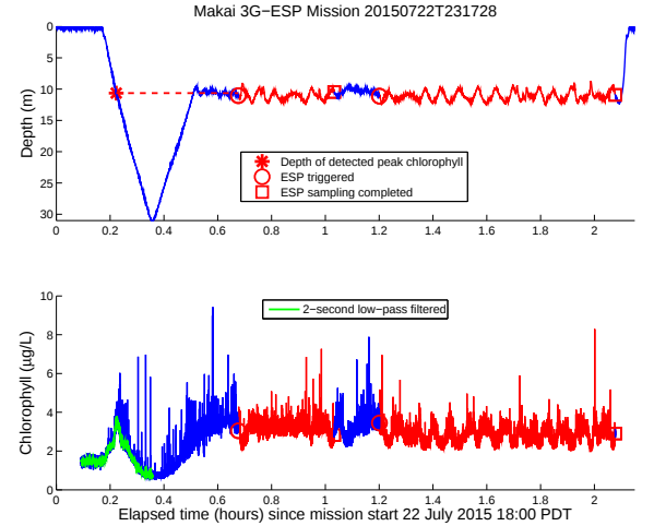
Fig. 5. The AUV's depth and chlorophyll measurements during the first peak detection and sampling mission. The low-pass filtered chlorophyll signal Chl_{lp} is shown in green in the lower panel. The peak-chlorophyll detection point is marked by the asterisk in the upper panel. The starting and ending points of the two ESP samplings are marked in both panels.
