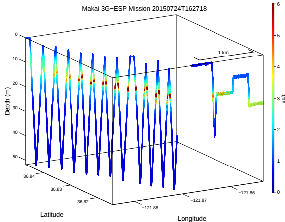
Fig. 6. The Makai AUV's initial yo-yo survey (left part), followed by the second autonomous peak detection and sampling mission (right part).
