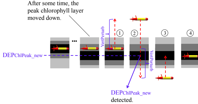
Fig. 3. Illustration of the algorithm for reacquiring the peak-chlorophyll layer when it moves down.
