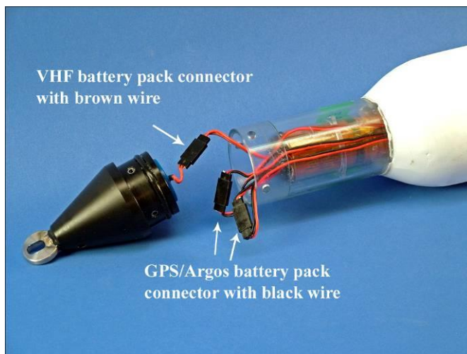
Fig. 2 Battery packs ready to be disconnected from TMT-464-2 and TMT-464-3
