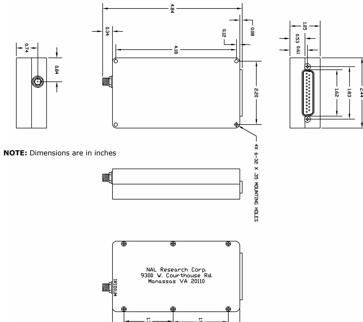
Figure 2. Mechanical drawings of model 9601-D-N.
