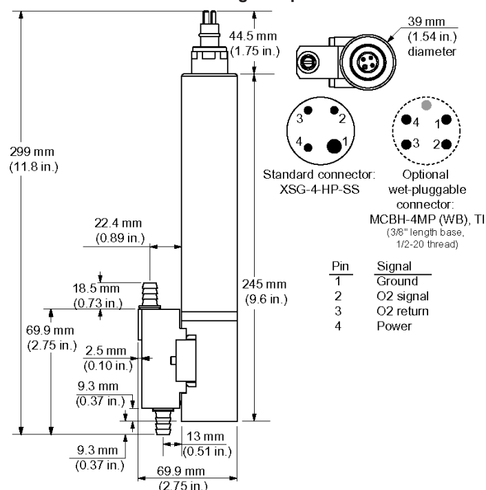
SBE 43 Voltage Output Sensor
