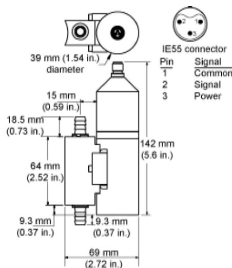
SBE 43F Frequency Output Sensor (for 52-MP, Glider Payload CTD, & OEM applications)
