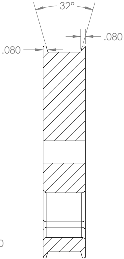
SECTION C-C
