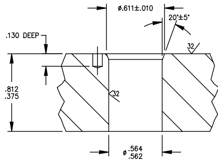
THROUGH BORE OPTION SECTION A-A
