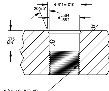
THREADED OPTION
