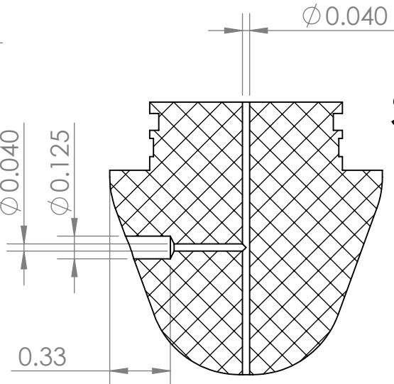
SECTION B-B SCALE 2 : 1.5
