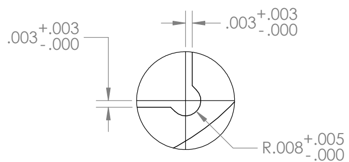
DETAIL C SCALE 20 : 1
