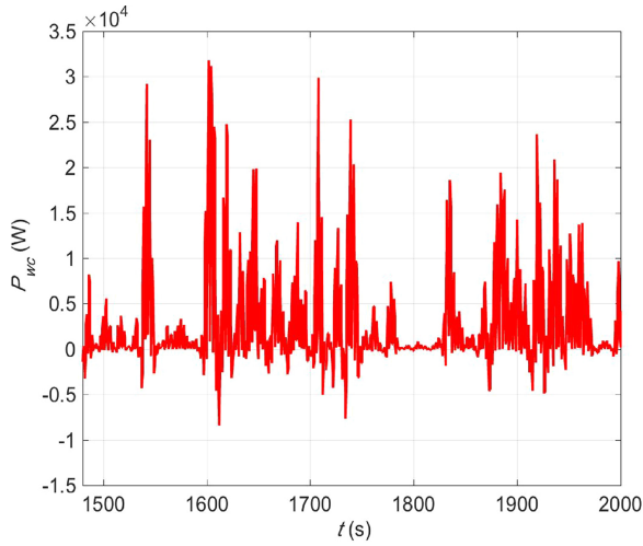
Fig. 4. The converted power time series for the test conditions ( H_s = 1.0 m, T_e = 6.0 s) with the amplitude and phase-limit conditions as applied here.
