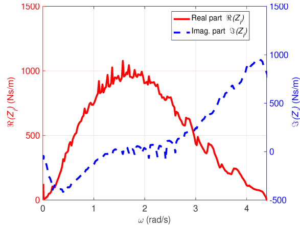
Fig. 14. Intrinsic impedance real and imaginary components for the equivalent single-body representing the 2-body coupled axi-symmetric system. Contributions of the in-air mass, infinite-frequency added mass, and hydrostatic stiffness are not included. The rapid undulations are likely due to interpolation errors introduced because the frequency-increment in the original data from the software calculations [19] was greater than that used in the present work.
