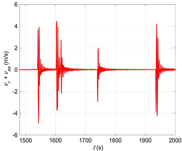
Fig. 6. The relative heave velocity time series, as resulting from end-stop impacts for the test conditions ( H_s = 1.0 m, T_e = 6.0 s) with the amplitude and phase-limit conditions as applied here. This is the time series without superimposing the wave-induced velocity time series.
