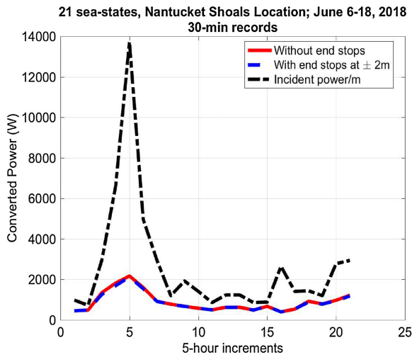
Fig. 10. Overview of power conversion for the various sea-states tested in this work under amplitude and phase-limit conditions. Note that conversion is close to maximum in the less energetic spectra, as desired, while the constraints lead to a significantly smaller converted power relative to the average incident power.
