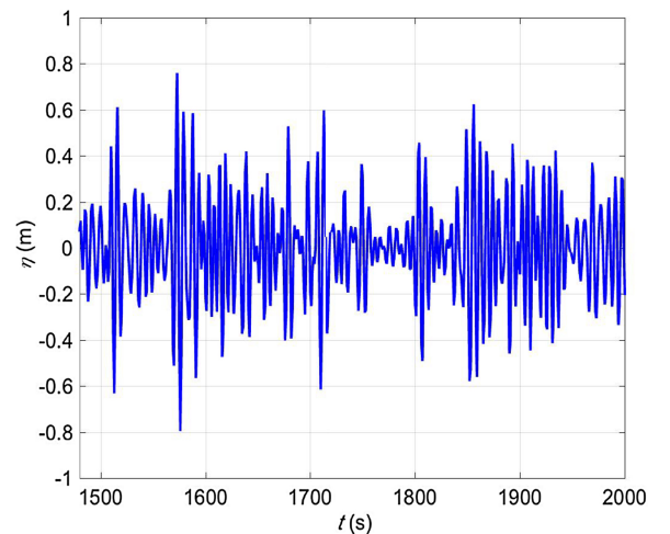
Fig. 3. The predicted wave elevation time series for the test conditions ( H_s = 1.0 m, T_e = 6.0 s) at prediction time t_p = 30 s, obtained as summarized in Appendix 2.
