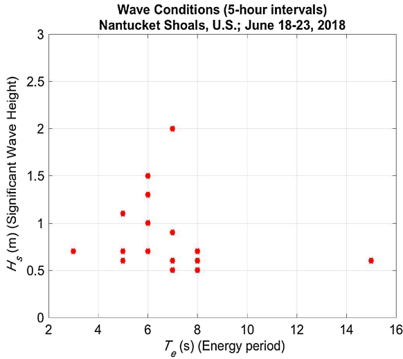
Fig. 2. Plot showing the energy period and significant wave height combinations observed at the site off the U.S. east coast.
