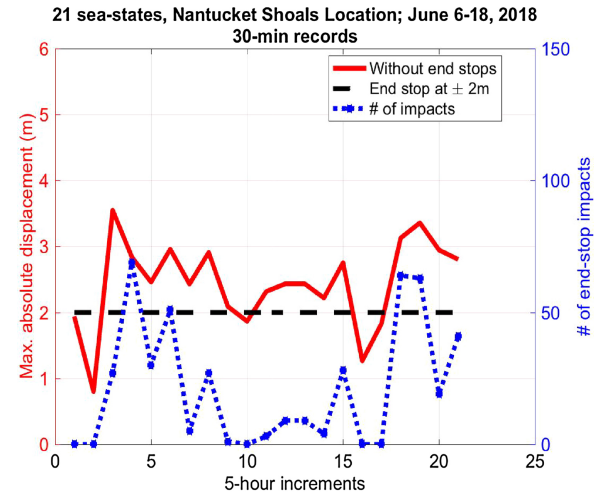
Fig. 11. Overview of the 30-min maximum displacement in the various sea-states tested in this work under amplitude and phase-limit conditions. Also shown is the number of times end-stop collisions occur during each 30-min simulation.
