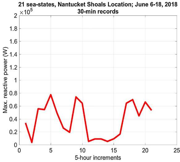
Fig. 13. Overview of the 30-min maximum reactive power in the various sea-states tested in this work under amplitude and phase-limit conditions.
