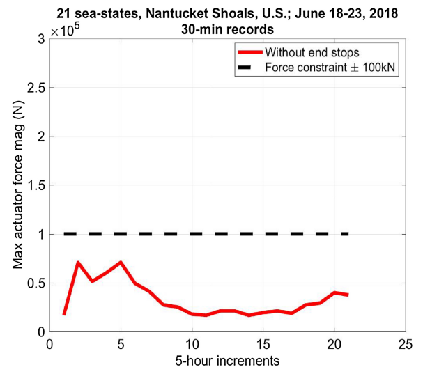
Fig. 12. Overview of the 30-min maximum force in the various sea-states tested in this work under amplitude and phase-limit conditions. The forces are seen to be within the imposed constraints.
