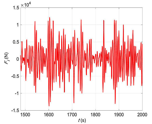
Fig. 8. The resistive force time series required for the test conditions ( H_s = 1.0 m, T_e = 6.0 s) with the amplitude and phase-limit conditions as applied here.
