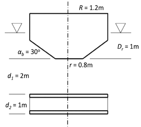
Fig. 1. The 2-body axisymmetric converter studied in this work. Relative heave oscillation is used in energy conversion, and the equations of motion can be rearranged in terms of the relative oscillation so that the relative heave dynamics can be understood using a single-mode framework. The buoy radius matches that of a mid-size oceanographic buoy. The space between the two submerged concentric discs may be used to support oceanographic sensors.
