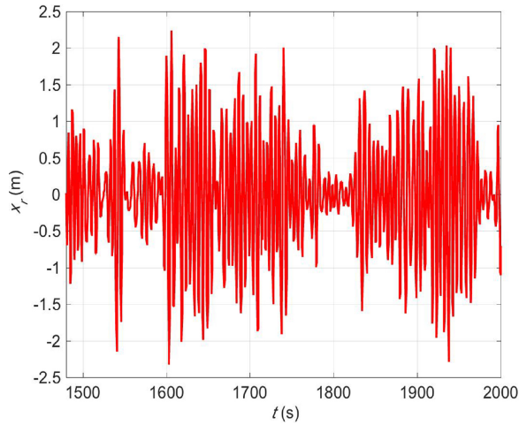
Fig. 5. The relative heave displacement time series for the test conditions ( H_s = 1.0 m, T_e = 6.0 s) with the amplitude and phase-limit conditions as applied here.
