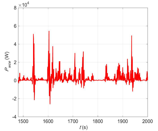
Fig. 7. The converted power time series with end-stop impacts occurring, for the test conditions ( H_s = 1.0 m, T_e = 6.0 s) with the amplitude and phase-limit conditions as applied here.
