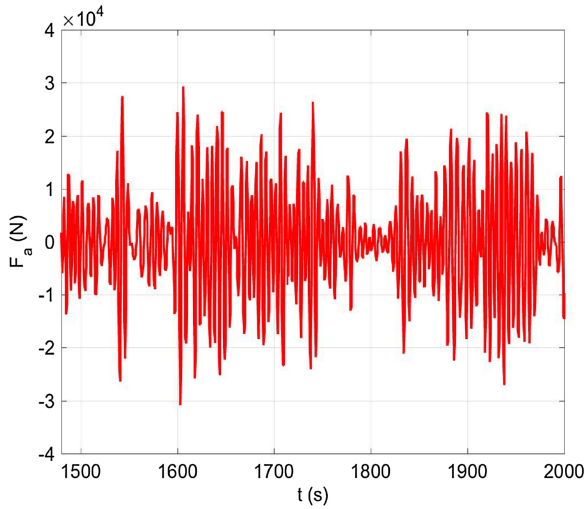
Fig. 9. The reactive force time series required for the test conditions ( H_s = 1.0 m, T_e = 6.0 s) with the amplitude and phase-limit conditions as applied here.
