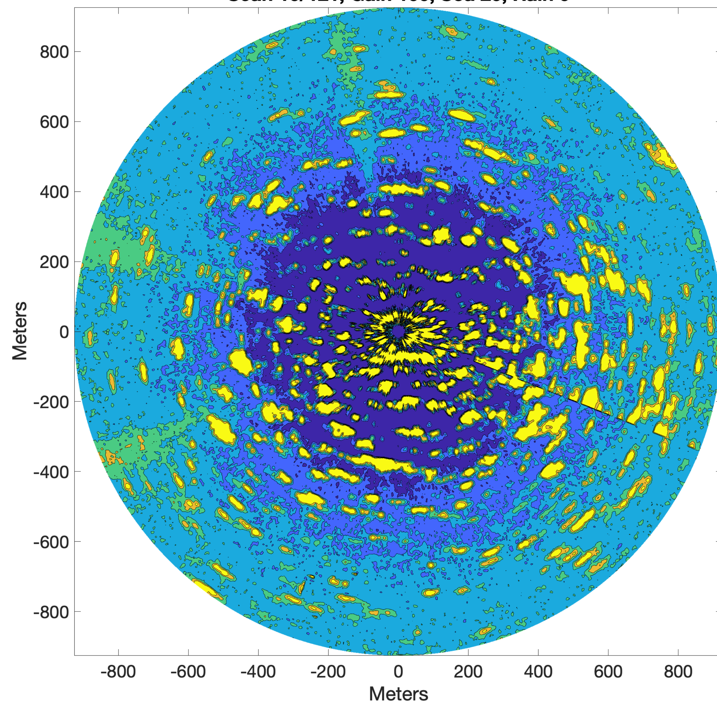
Scan 10/121, Gain 100, Sea 20, Rain 0
