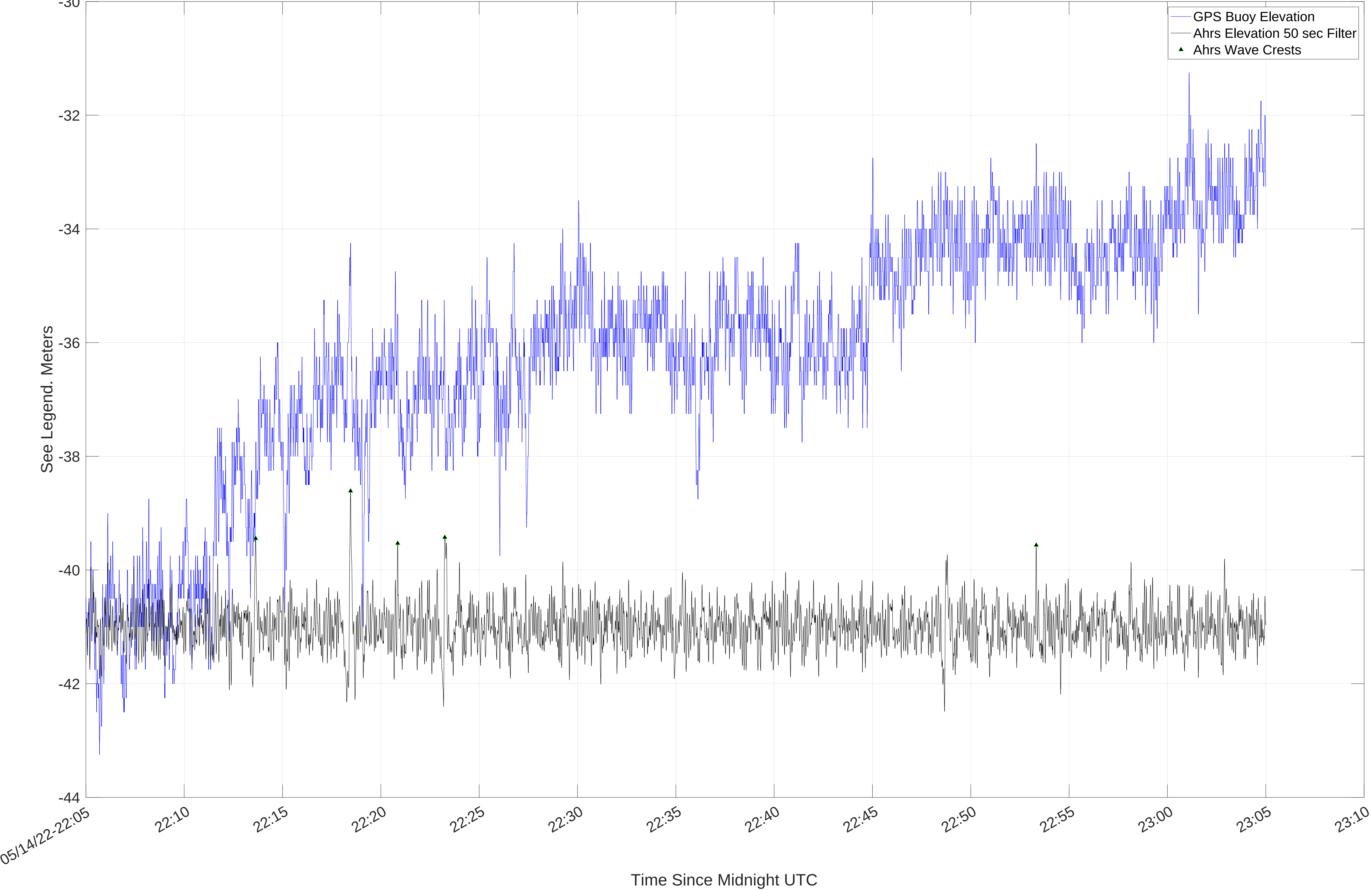
GPS/Ahrs Sea Surface and Elevation for Data Set 1652568771 (14-May-2022 22:52:51). H_{m0} = 1.5 m.
