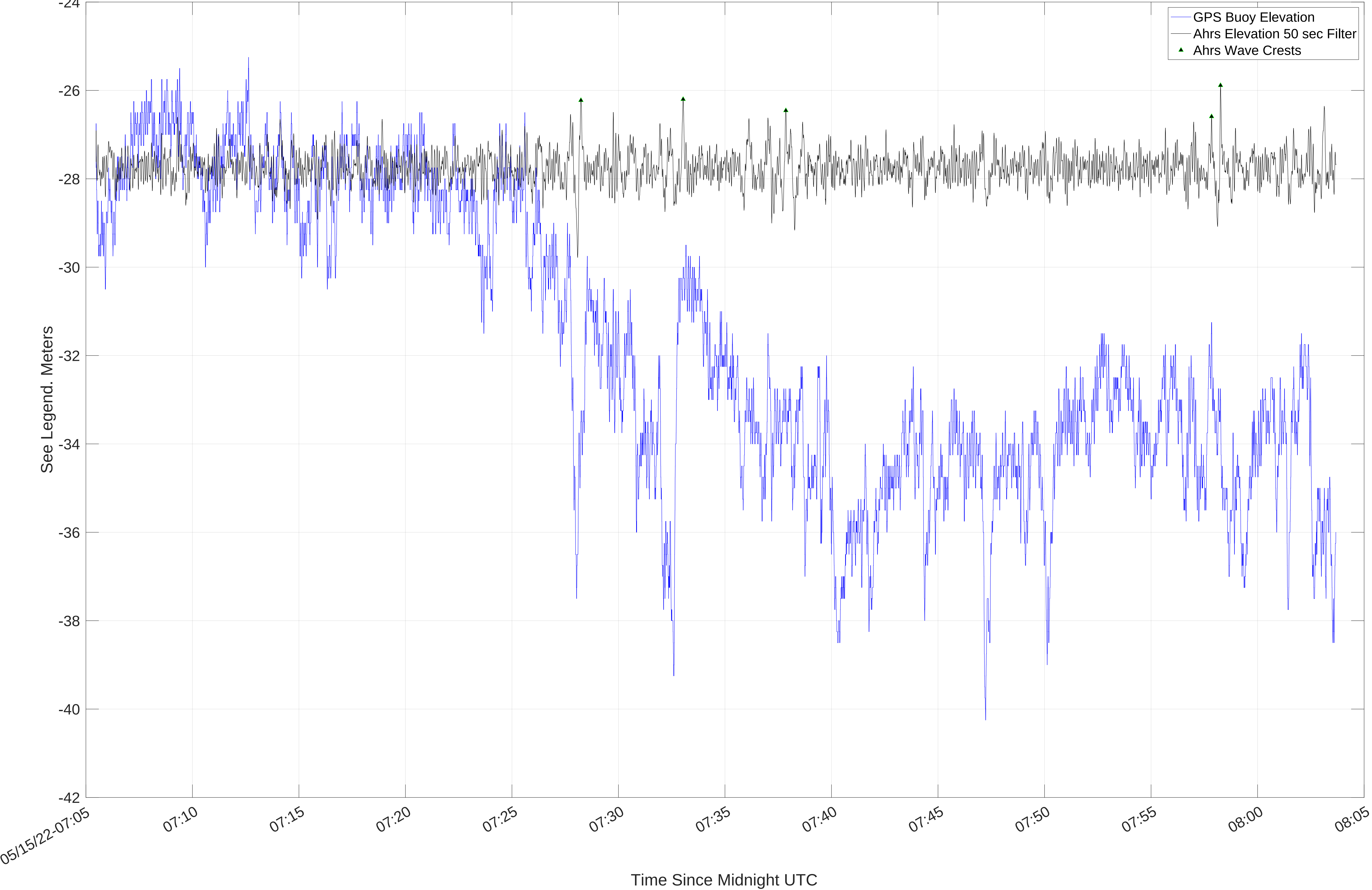
GPS/Ahrs Sea Surface and Elevation for Data Set 1652598563 (15-May-2022 07:09:23). H_{m0} = 1.5 m.
