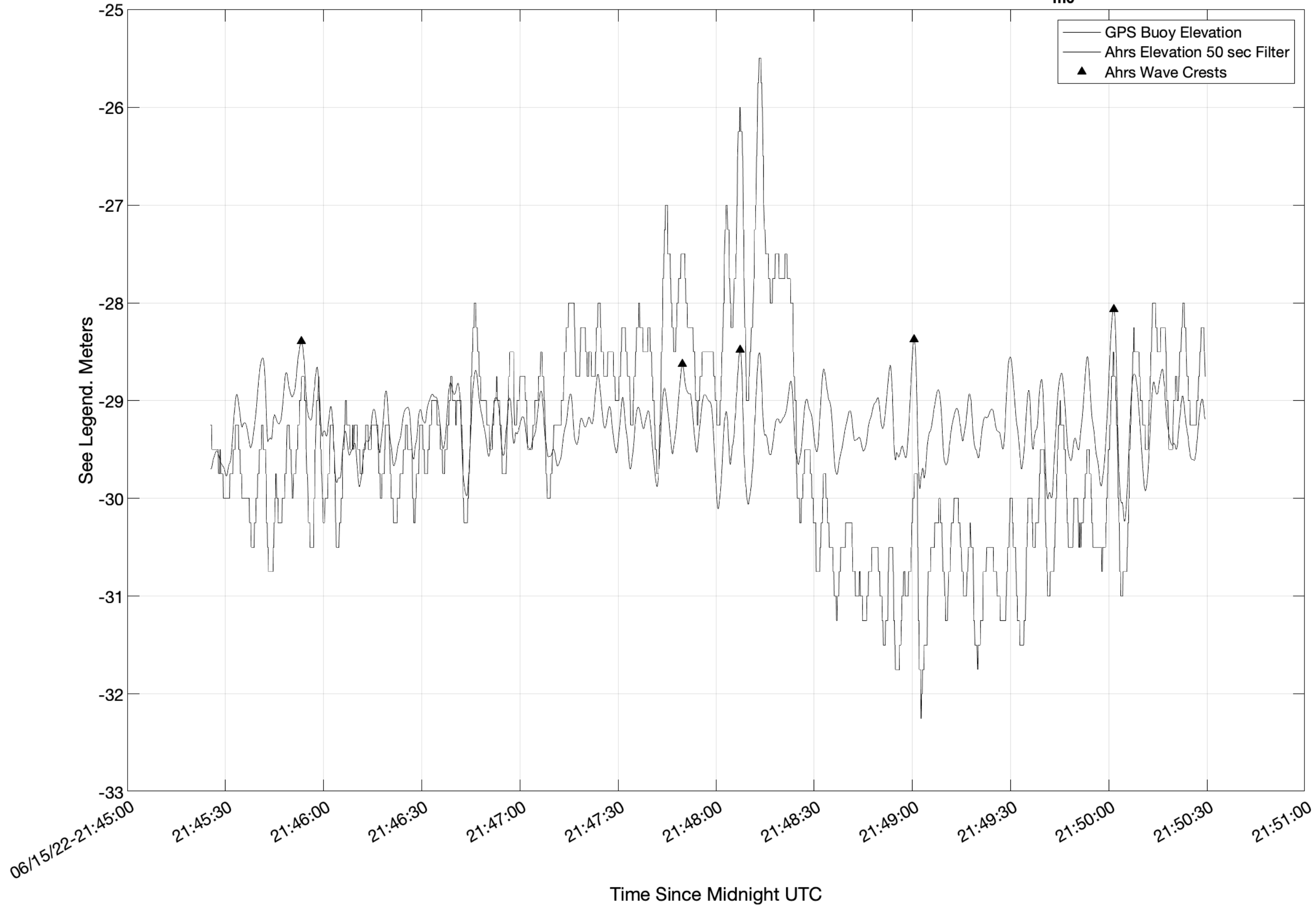
GPS/Ahrs Sea Surface and Elevation for Data Set 1655329829 (15-Jun-2022 21:50:29). H_{m0} = 1.3 m.
