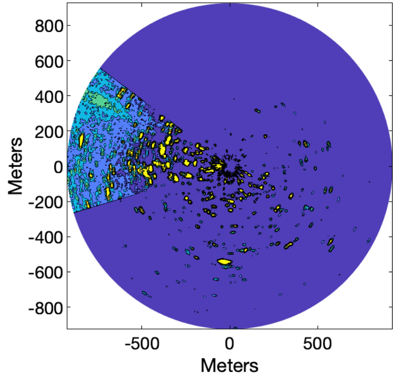
Scan 80/121, Dur 2.432 sec, Gain 80100, Sea 40, Rain 0
