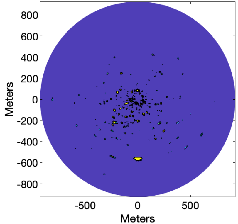
Scan 78/121, Dur 2.502 sec, Gain 80, Sea 40, Rain 0
