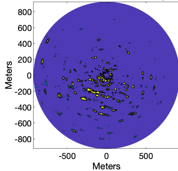
Scan 98/121, Gain 90, Sea 70, Rain 0
