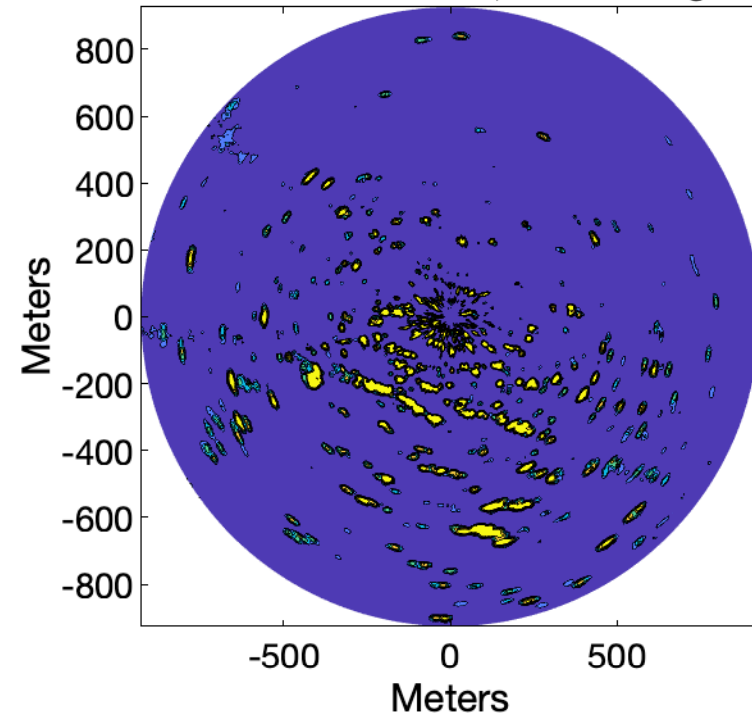
Scan 95/121, Gain 90, Sea 70, Rain 0
