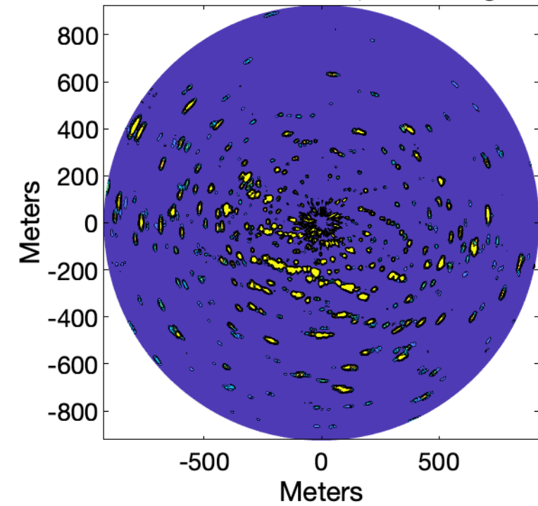
Scan 100/121, Gain 90, Sea 70050, Rain 0
